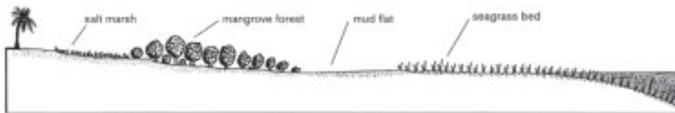
Figure 5. Cross section of a typical sheltered shore showing the main habitats during low tide.
